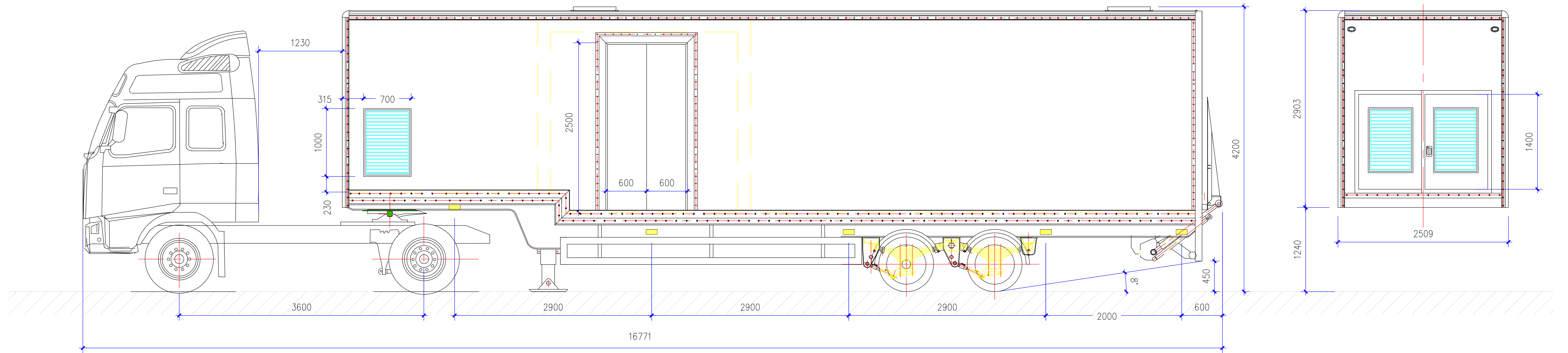
A - A SECTION
